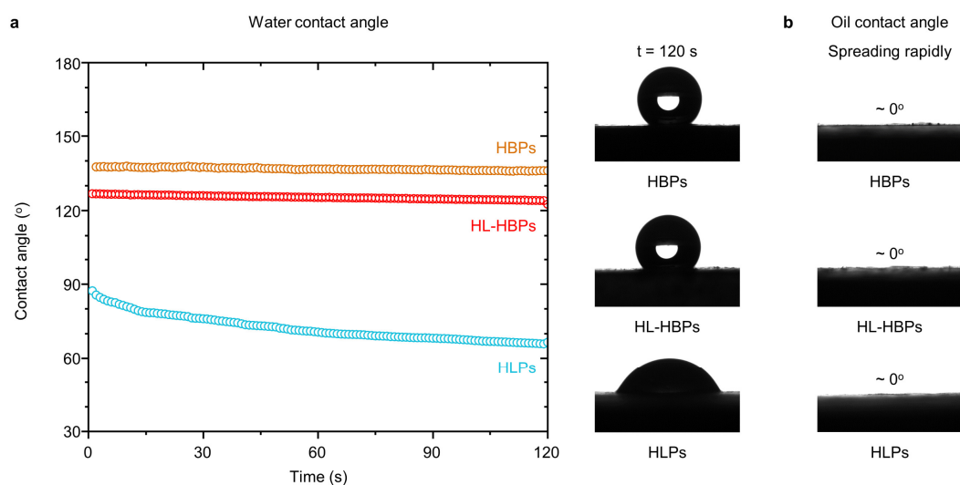
Supplementary Fig. 6. Contact angle measurement of HL-HBPs, HLPs, and HBPs. a , Time-lapse water contact angle measurement in air. The HBPs show a relatively hydrophobic nature, with contact angle of 136.0 \pm 2.7^\circ at 120 s. The HLPs show a relatively hydrophilic nature, with contact angle of 66.5 \pm 0.4^\circ at 120 s. The HL-HBPs show a relatively hydrophilic nature compared with HBPs, and relatively hydrophobic nature compared with HLPs, with contact angle of 122.6 \pm 1.6^\circ at 120 s. These results suggest that the HL-HBPs are more favorable for water wetting compared with HBPs, facilitating their dispersion in water. Contact angle values: Mean \pm SD, n = 3 . b , Oil contact angle measurement in air. The oil droplets spread rapidly for all particles, probably due to the low interfacial tension of the oil (octane). Contact angle measurement process is described as follows. The particle powders were adhered to a tape on a glass slide. Powders that were not tightly adhered were blew away. A drop (2 \mu L) of water or oil (octane) was dropped on the particles. A surface analyzer (LSA 100, LAUDA Scientific, GmbH) was used to determine the contact angles. For water contact angle in air, the data were automatically calculated and recorded by the software. For oil contact angle in air, the oil droplets can spread rapidly with a contact angle of \sim 0^\circ . We would like to clarify that the contact angle for HL-HBPs adhered tape ( 122.6 \pm 1.6^\circ ) does not certainly imply the absence of electrostatic interaction on HL-HBPs. The hydrophilicity-hydrophobicity of the particles was evaluated by a commonly-used approach. Typically, the particles were adhered to a glass microscope slide by double-sided adhesive tape, and three-phase contact angle was measured by the sessile drop method 1 . The contact angle can be affected by the coverage of the particles on the tape, the interfacial tension of the
