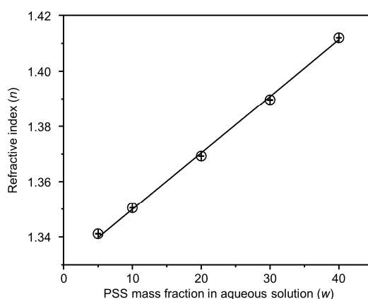
Supplementary Fig. 8. Relationship between refractive index ( n ) and PSS mass fraction ( w ) in aqueous solution. The refractive index ( n ) of pure PSS was predicted by measuring the refractive indices of PSS aqueous solutions with different PSS mass fraction ( w ). A series of PSS (average M_w = 70000 , purchased from Sigma Aldrich) aqueous solutions were prepared with PSS mass fraction of 5%, 10%, 20%, 30%, and 40%, respectively. Subsequently, their refractive indices were measured with an Abbe refractometer at 20 °C ( n_{20/D} ) (Mean \pm SD, n = 3 ). The relationship between n and w can be linearly fitted 8 with an equation of n = 0.00204 \times w + 1.3295 ( R^2 = 0.99881 ). When pure PSS is applied ( w = 100\% ), n = 1.5335 , which is in accordance with previous study 9 .
